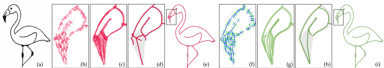
Figure 1: For a given bitmap image (a), state-of-the-art line drawing vectorization algorithms [BS19, SBBB20, PNCB21] rely on frame fields (b) aligned with the curve directions in the image. In [BS19], for instance, those are used to trace streamlines (c), leading to the final vectorization (d,e). We develop a novel framework producing singularity-free frame fields, which can be combed globally (f), allowing for a more robust resolution of directions of intersecting curves, better streamlines (g), and ultimately, better vectorization (h,i) without changing the rest of the vectorization algorithm. Input image ©Tracie Kiernan, https://stepbystepainting.net/ .
