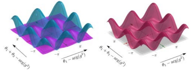
Figure 5: Regularizing effect of E_v . The left graph shows the summand terms for a pixel in Eq. (12), with the product term in blue (taller peaks) and E_v in magenta (lower peaks, with an exaggerated v = 0.4 weight). The right graph shows the resulting sum E_{\text{Alignment}} in red, with clearly non-degenerate minima. Graphs created with the GeoGebra graphing application [HBA*23].
